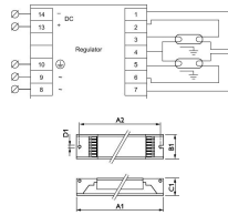
Specificaties Philips HF-R 236 TL-D EII 220-240V
